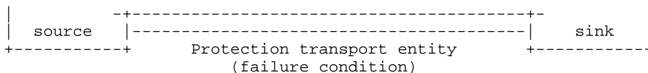
Figure 1: 1+1 unidirectional linear protection switching
