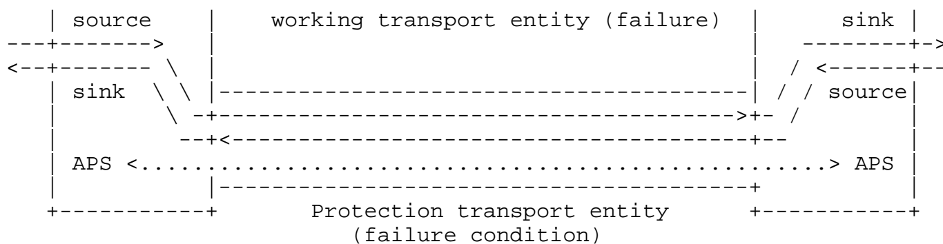
Figure 3: 1:1 bidirectional linear protection switching
