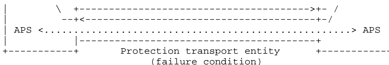
Figure 2: 1+1 bidirectional linear protection switching
