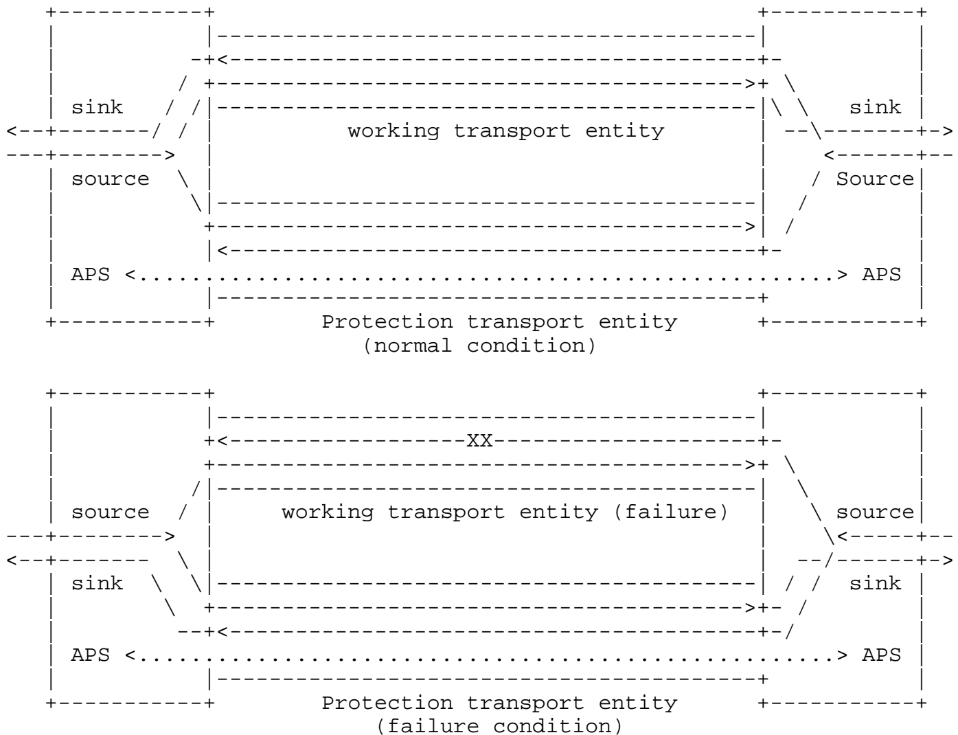
Figure 2: 1+1 bidirectional linear protection switching
