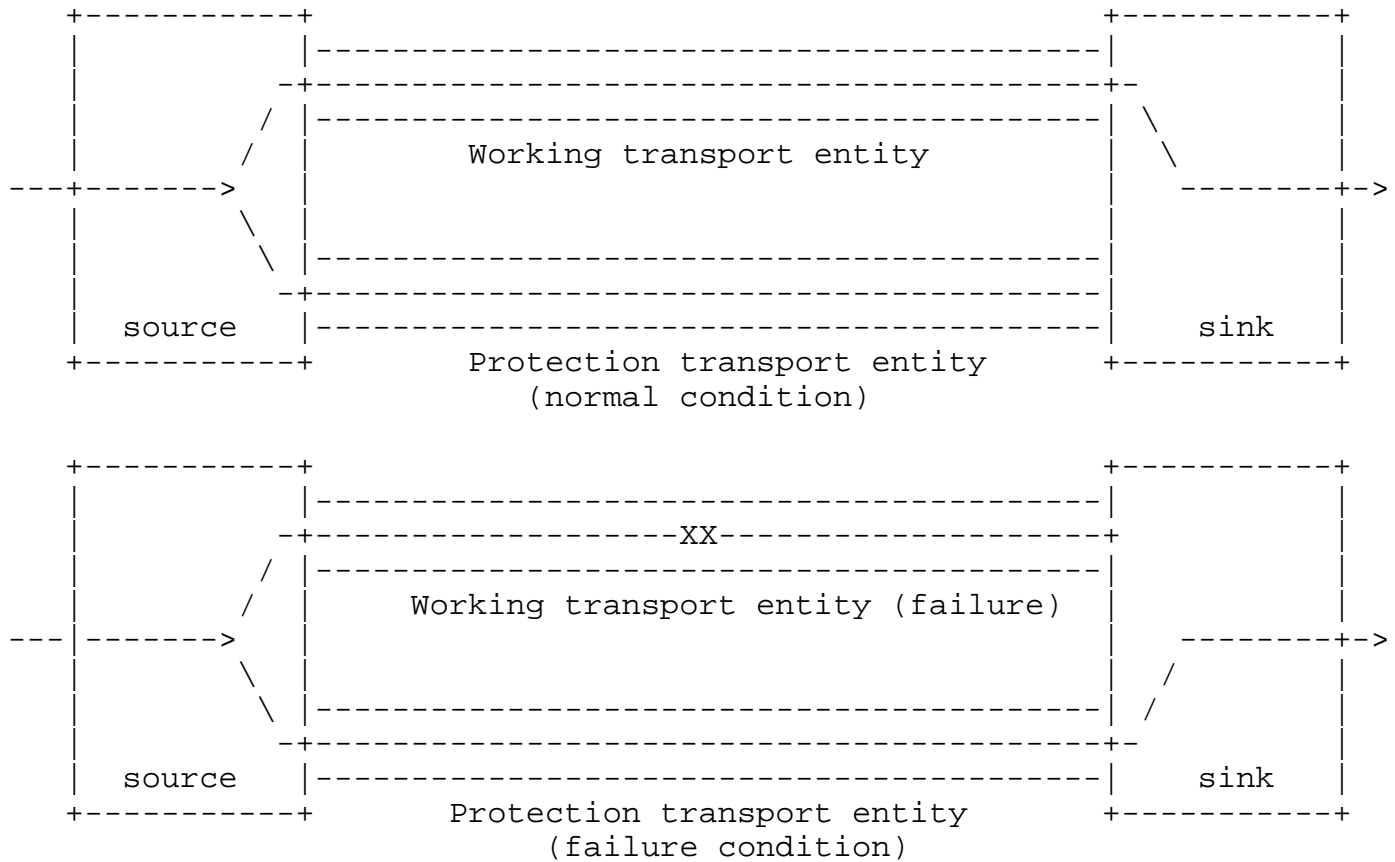
Figure 1: 1+1 unidirectional linear protection switching
