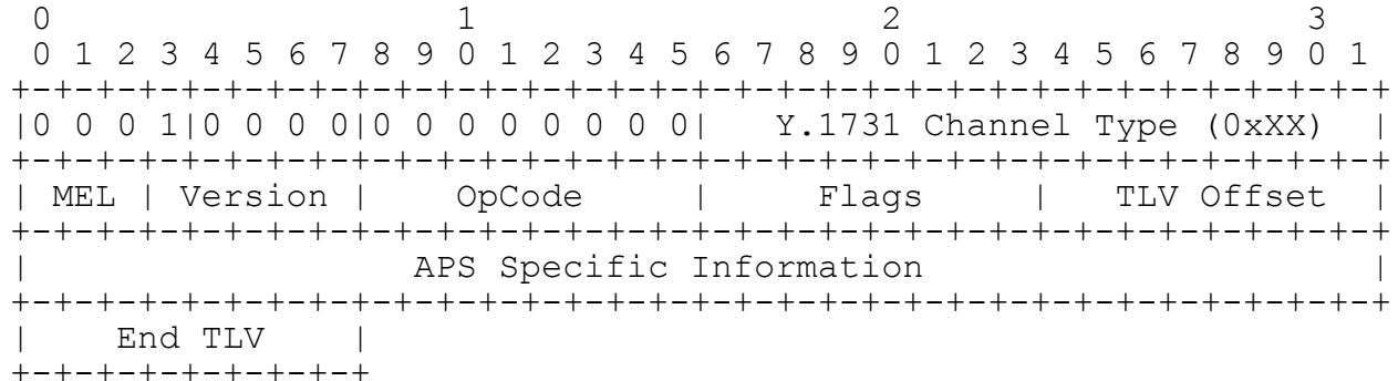
Figure 4 APS PDU format
