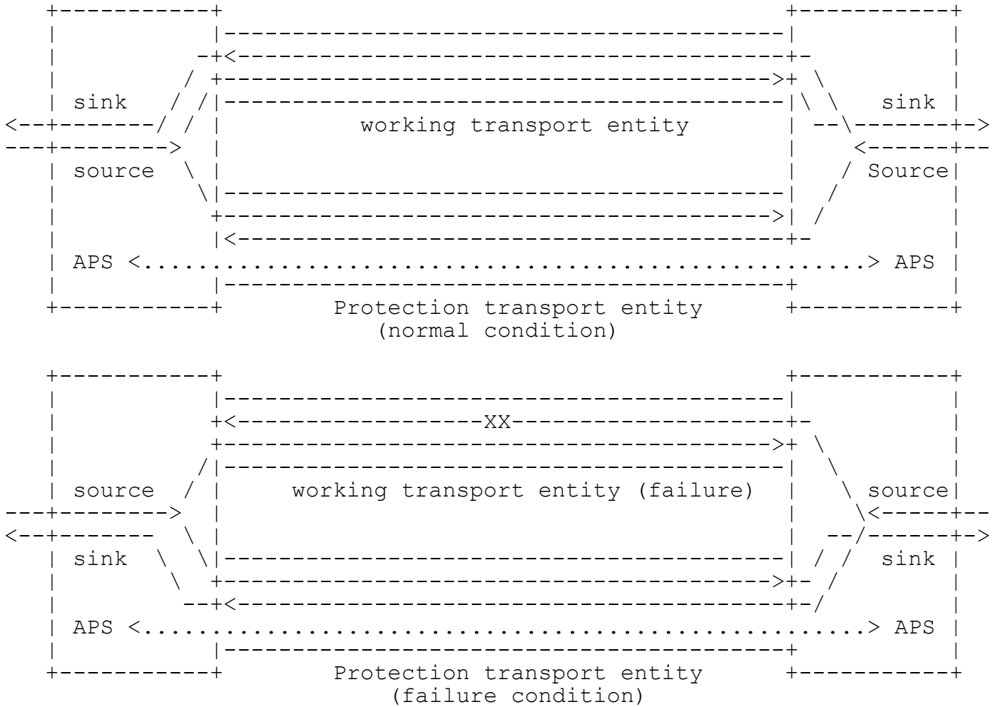
Figure 2 1+1 Bidirectional Linear Protection Switching
