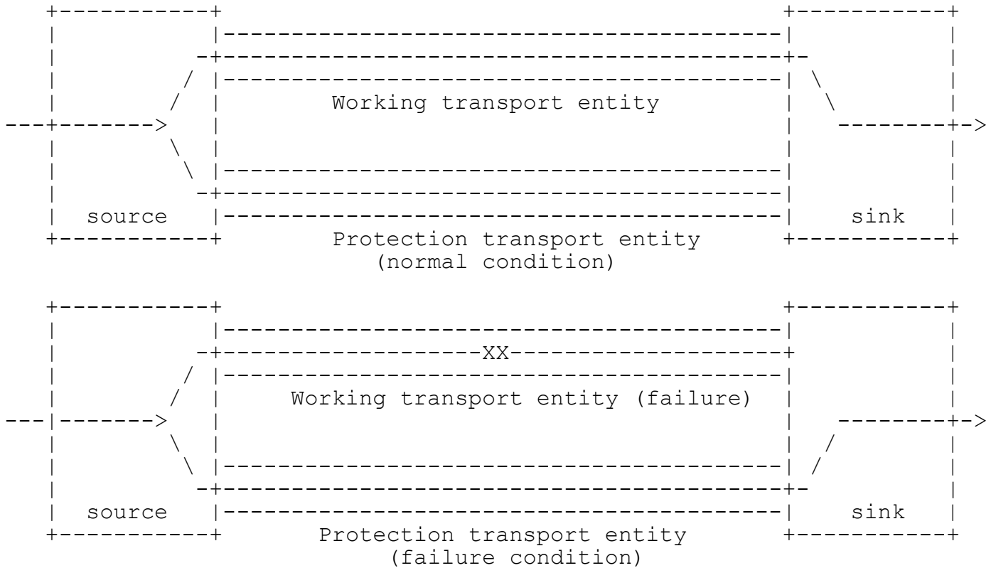
Figure 1 1+1 Unidirectional Linear Protection Switching
