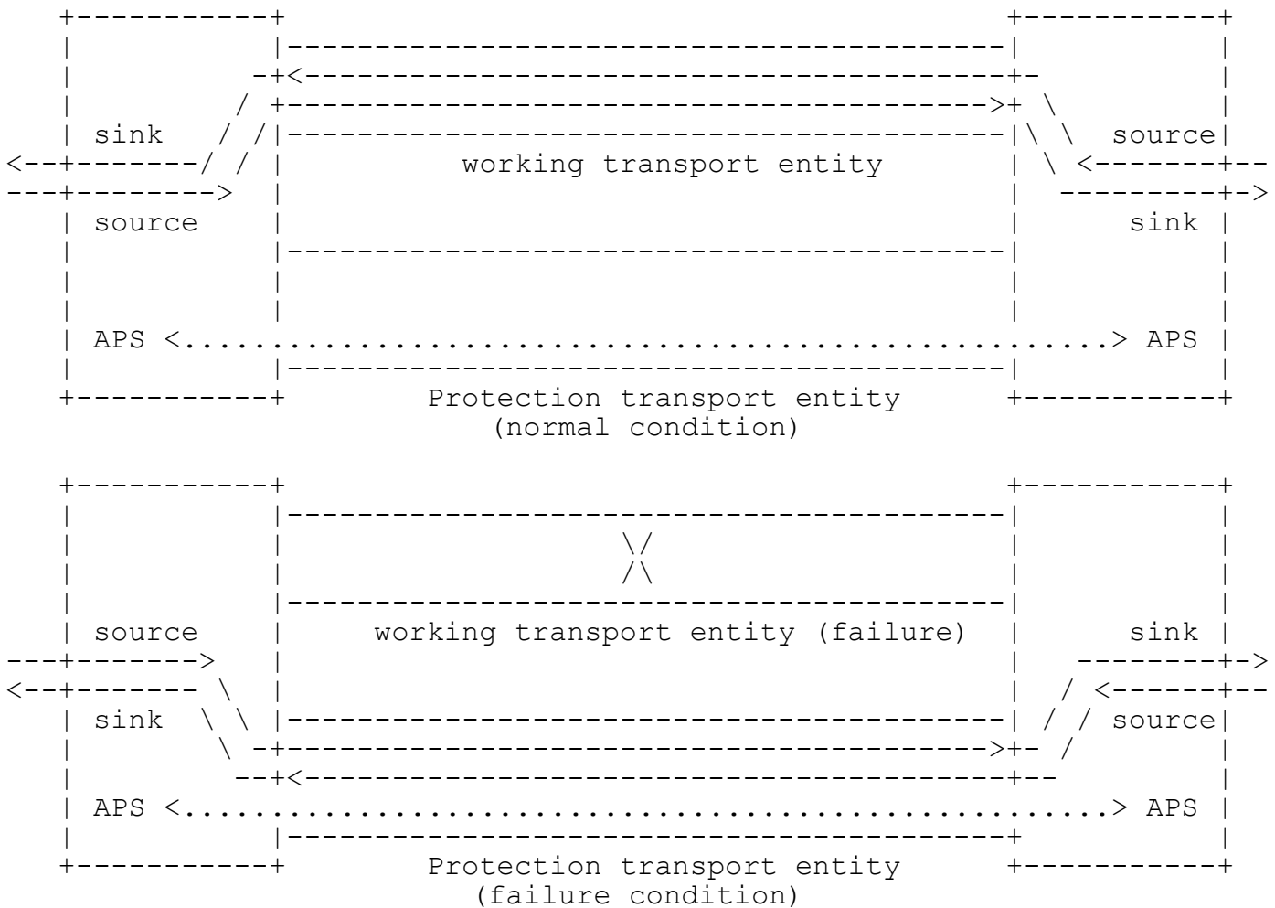
Figure 3 1:1 Bidirectional Linear Protection Switching
