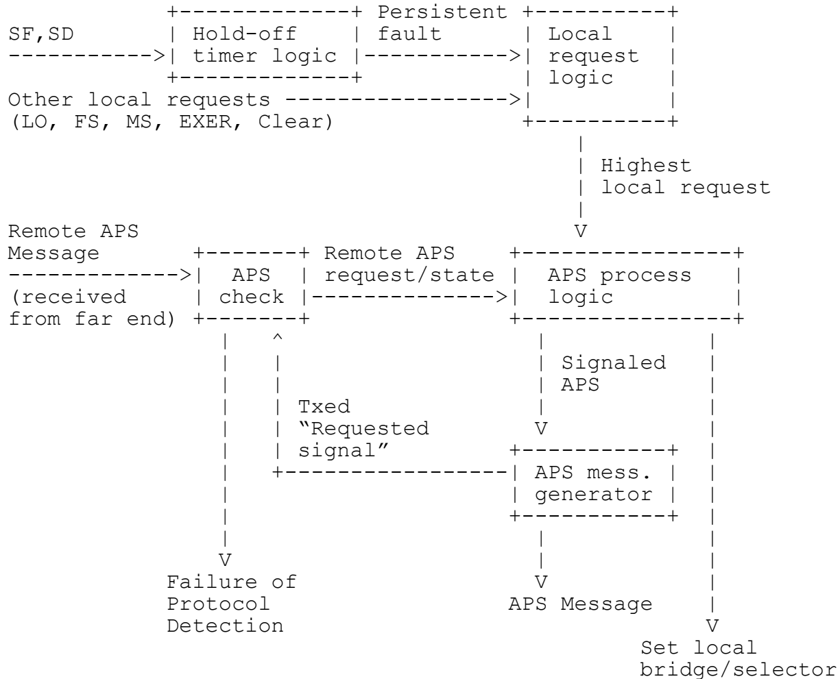
Figure 7 Protection Switching Logic
