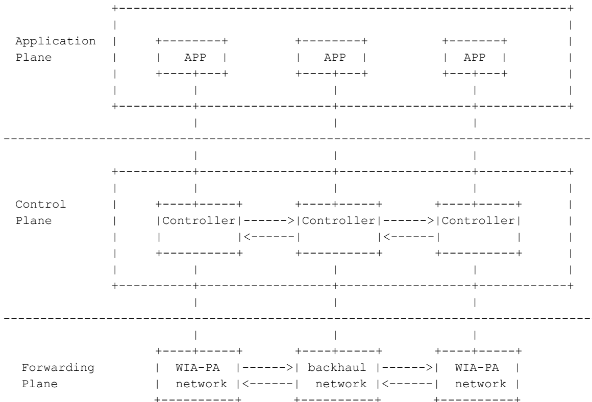
Figure 1. Distributed Architecture
