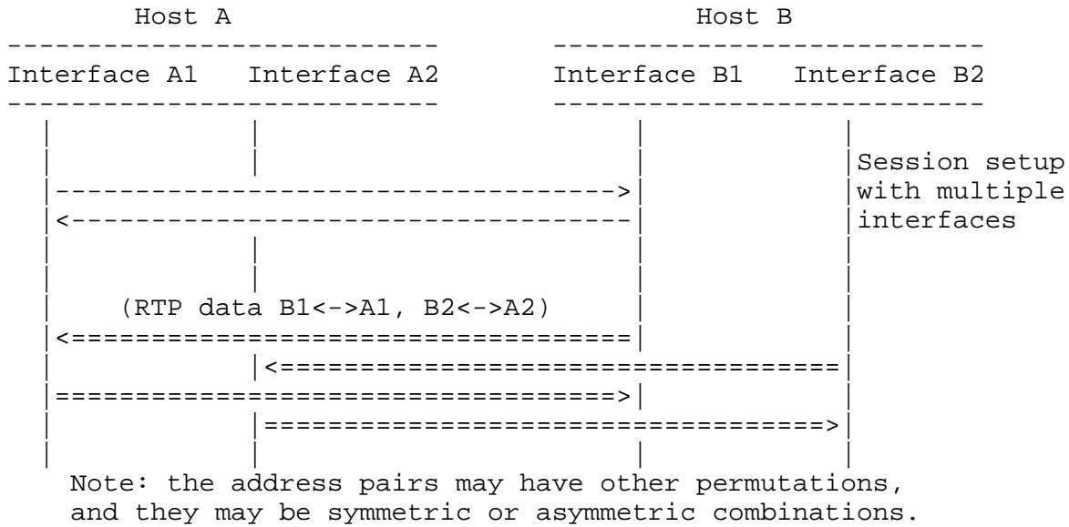
Figure 4: Bidirectional flow
