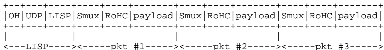
Figure 4: Structure of a LISP packet encapsulating three packets compressed with ROHC separated with Simplemux
