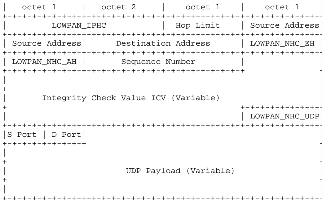
Figure 2: A sample NHC compressed IP/UDP packet secured with AH.
