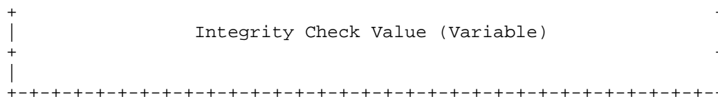
Figure 4: A sample NHC compressed IP/UDP packet secured with ESP.
