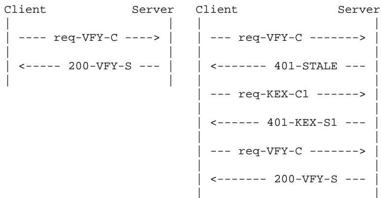
Figure 2: Several alternative flows on protocol
