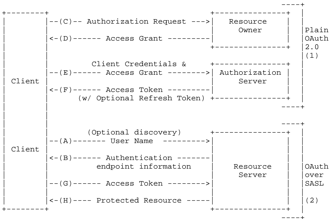
Figure 1: Interworking Architecture
