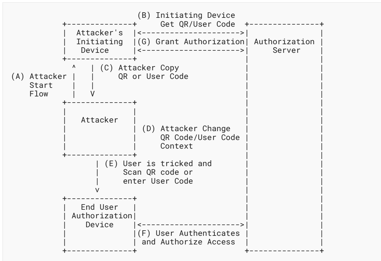
Figure 2: Attacker Initiated Cross Device Flow Exploit
