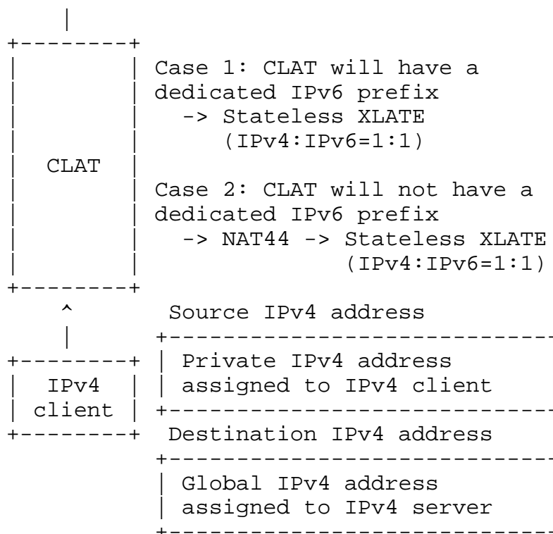
IPv4/IPv6 Address Translation Chart
