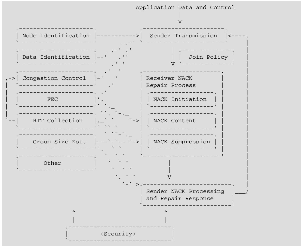
Figure 1: NACK-based Reliable Multicast Building Block Framework
