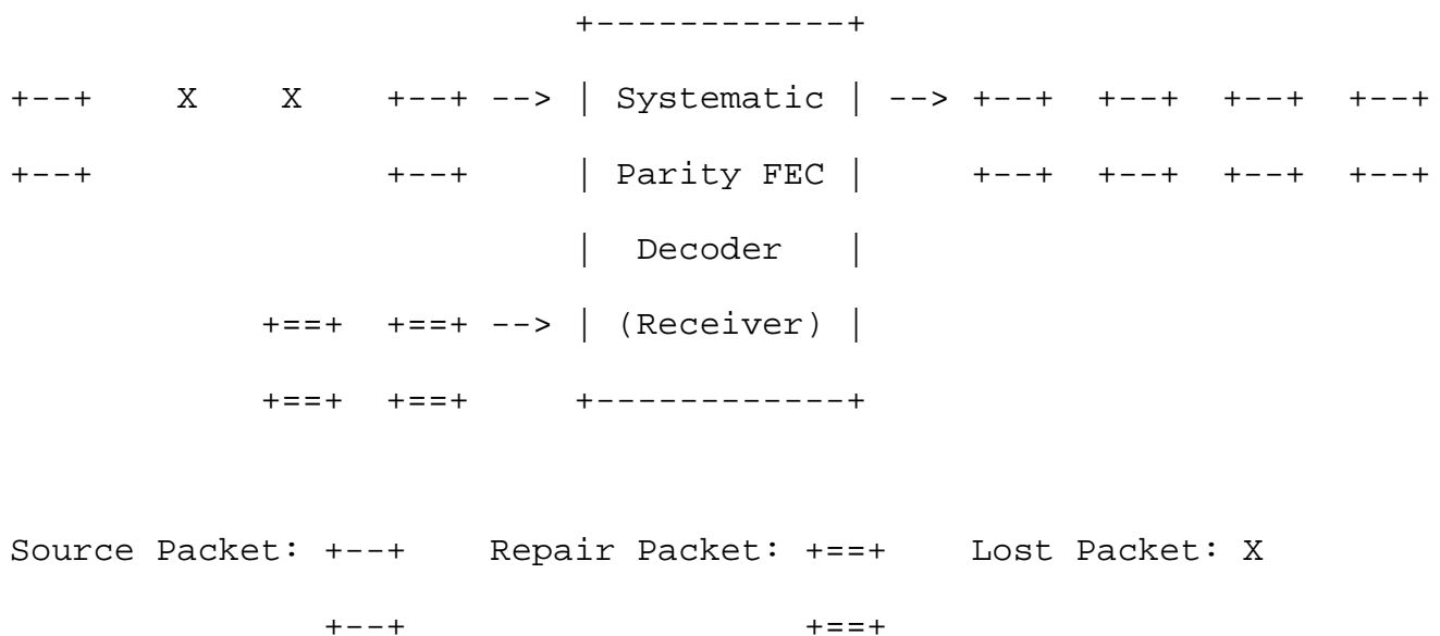
Figure 2: Block diagram for systematic parity FEC decoder
