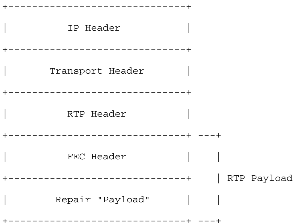
Figure 9: Format of FEC repair packets
