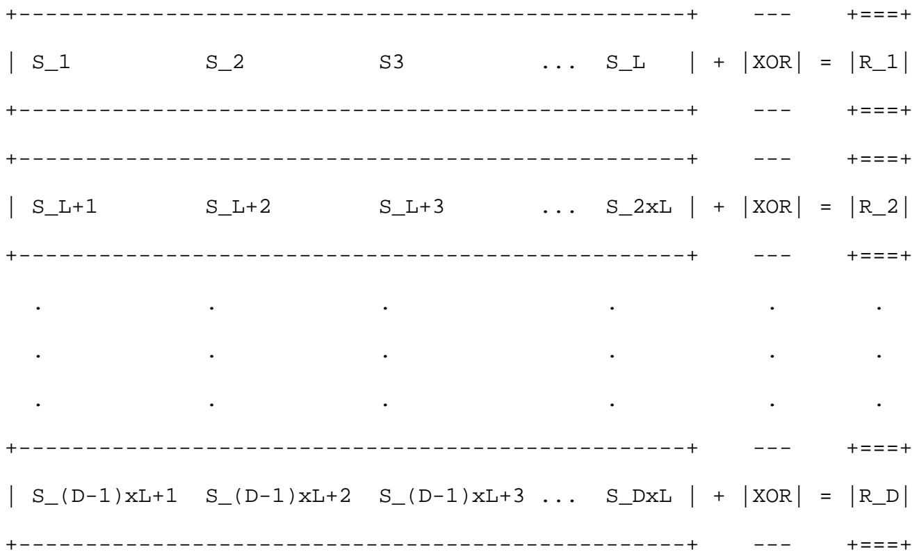
Figure 3: Generating non-interleaved (row) FEC repair packets
