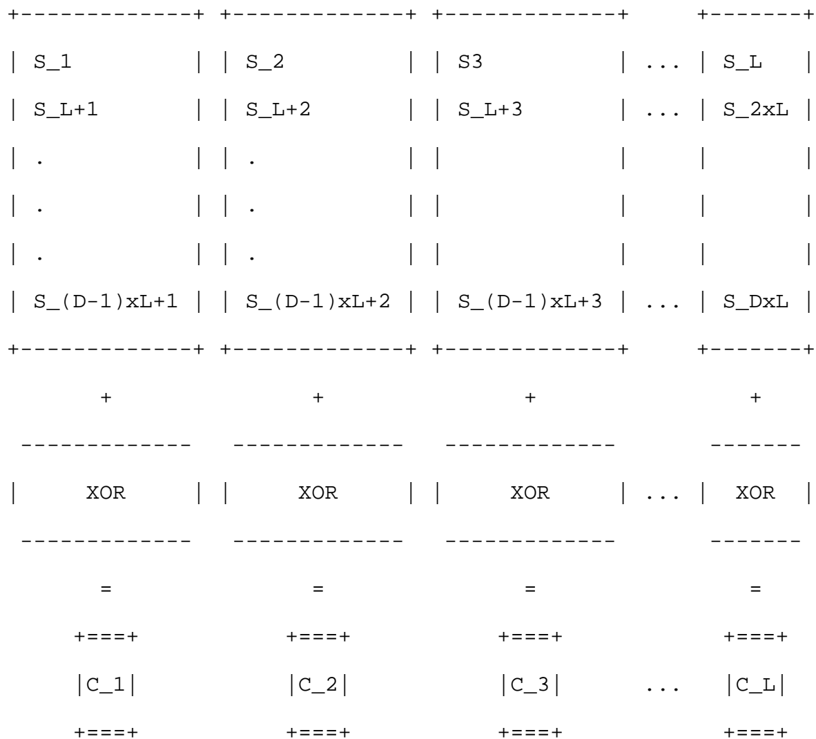
Figure 4: Generating interleaved (column) FEC repair packets
