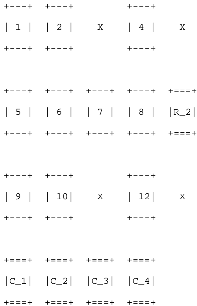
Figure 8: Example scenario #2 where 2-D parity FEC protection fails error recovery
