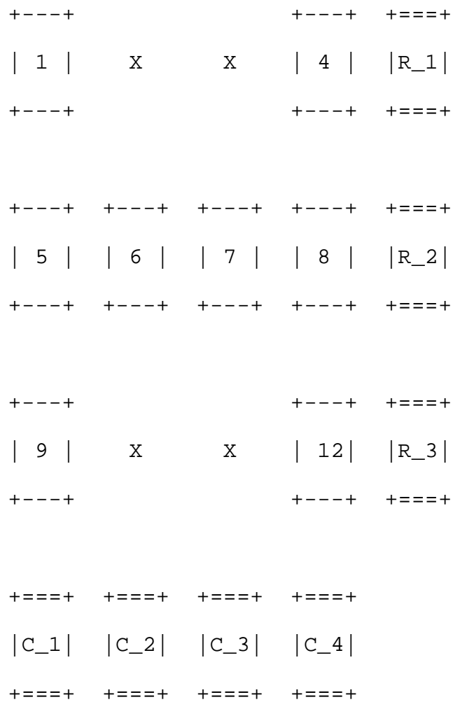
Figure 7: Example scenario #1 where 2-D parity FEC protection fails error recovery
