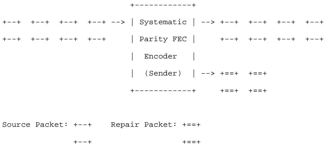
Figure 1: Block diagram for systematic parity FEC encoder
