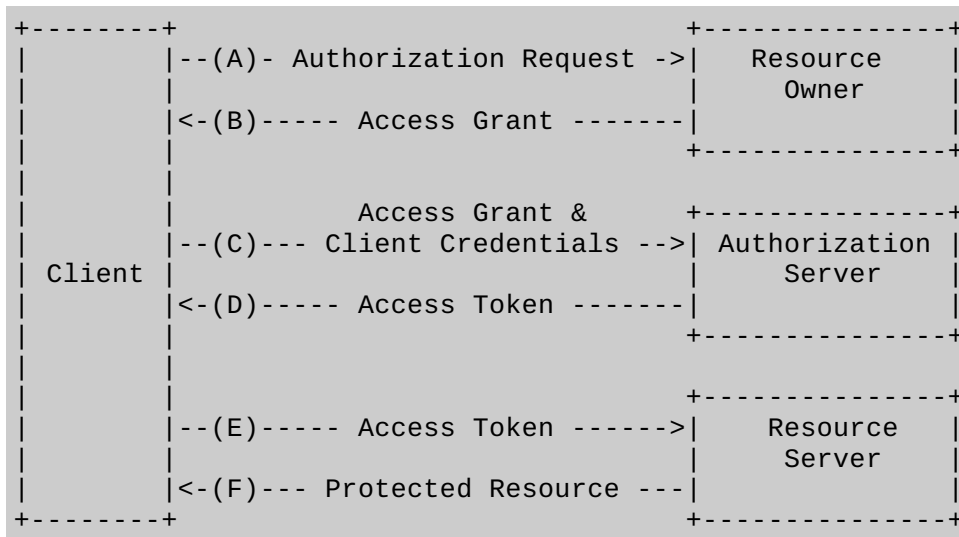
Figure 1: A Abstract Protocol Flow
