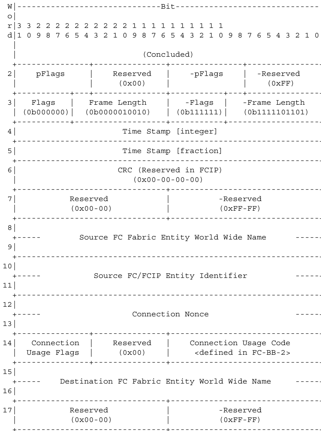
Fig. 9 FCIP Special Frame Format (part 2 of 2)
