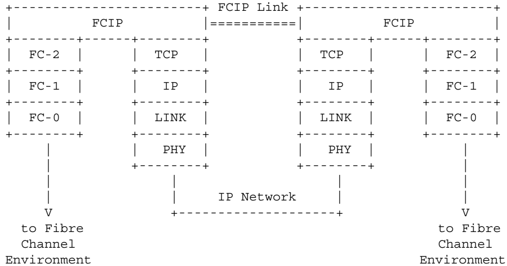
Fig. 1 FCIP Protocol Stack Model
