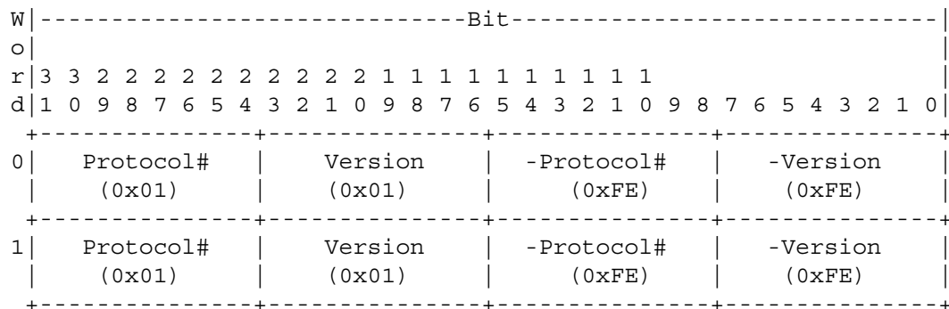
Fig. 9 FCIP Special Frame Format (part 1 of 2)
