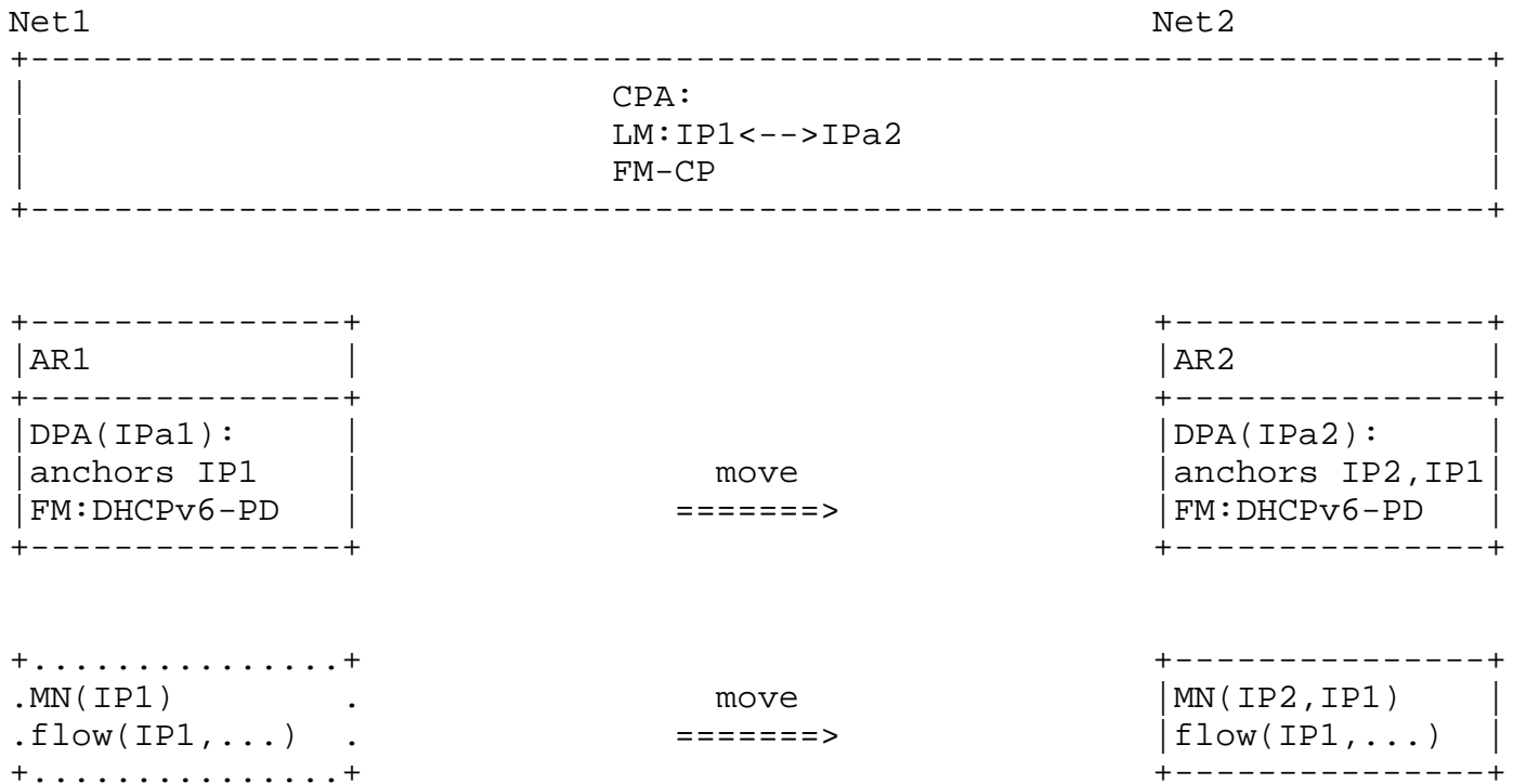
Figure 9. IP prefix/address anchor switching to the new network with LM and FM-CP in a centralized control plane whereas the FM-DP's are distributed.
