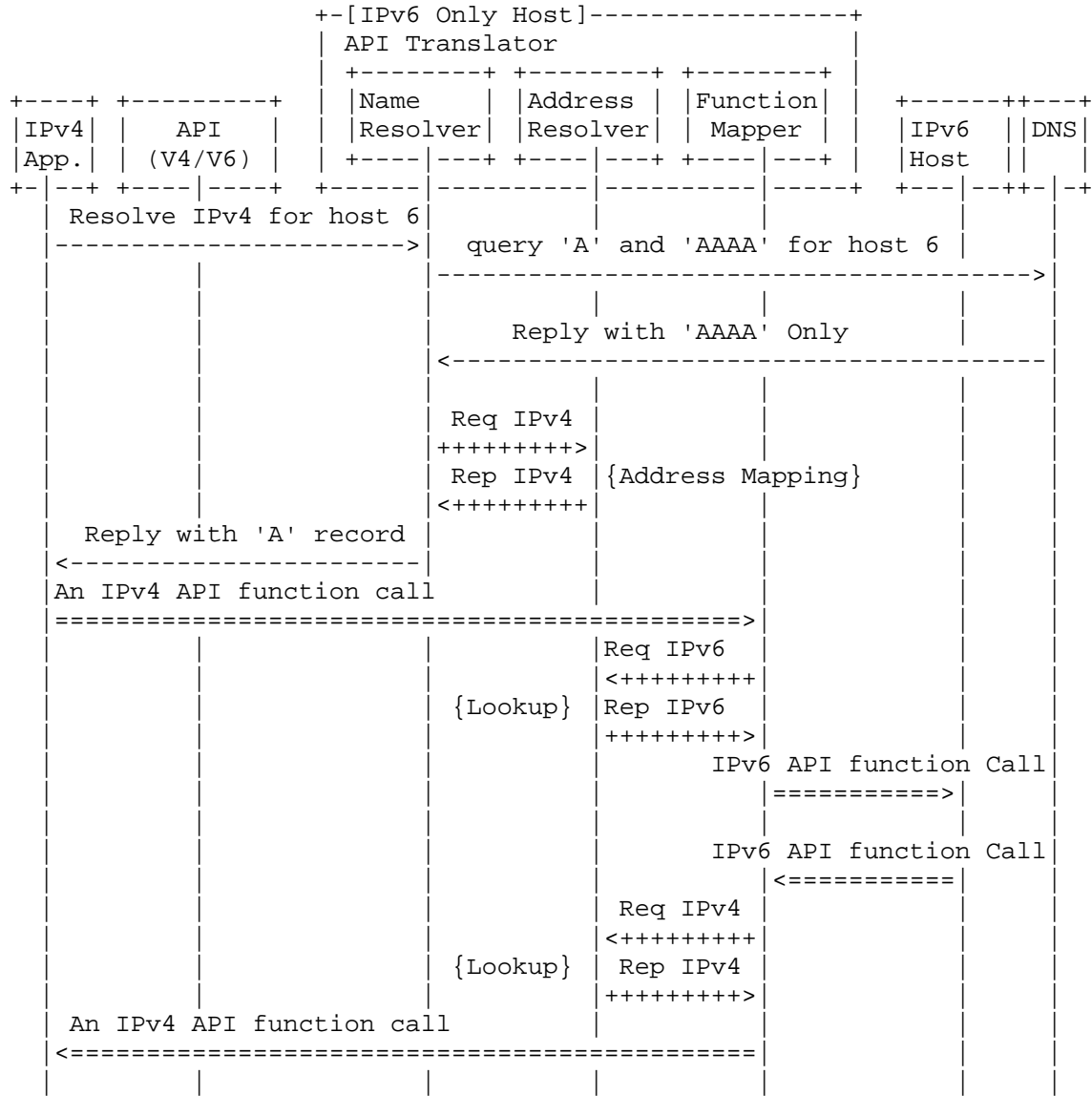
Figure 5: The behavior of the originator communicates with IPv6 Application
