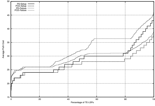
(a) Distribution of average path costs across TE-LSPs.
